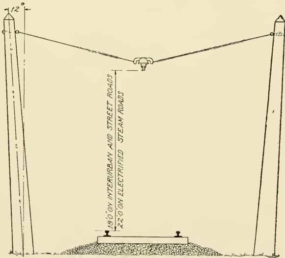
Fig. 191. Span Construction for Single Trolley Wire
